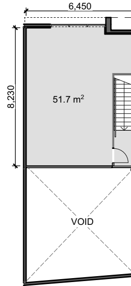
FIRST FLOOR PLAN 1:200 @ A4
