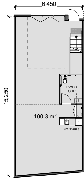
GROUND FLOOR PLAN 1:200 @ A4
