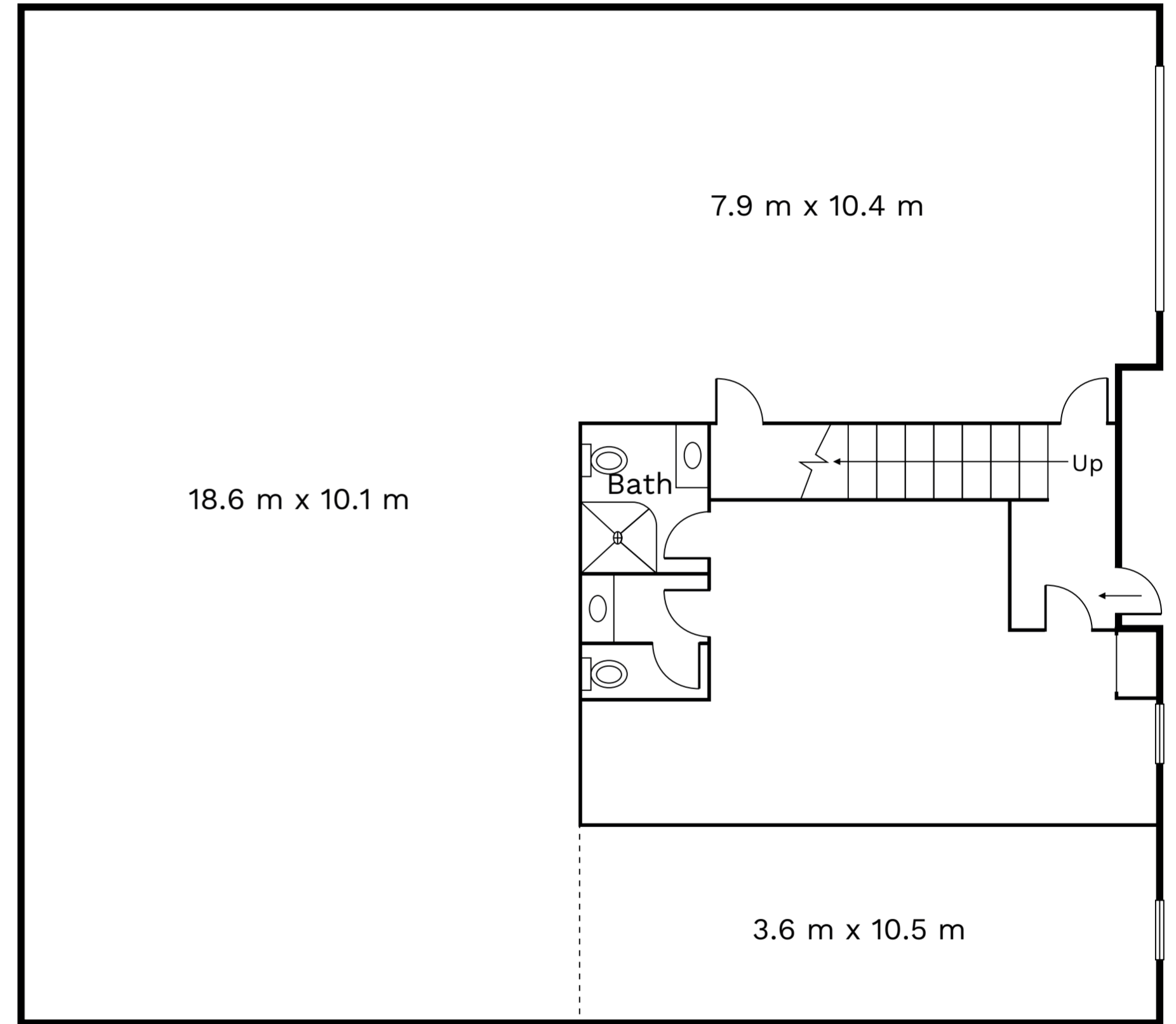
GROUND FLOOR
