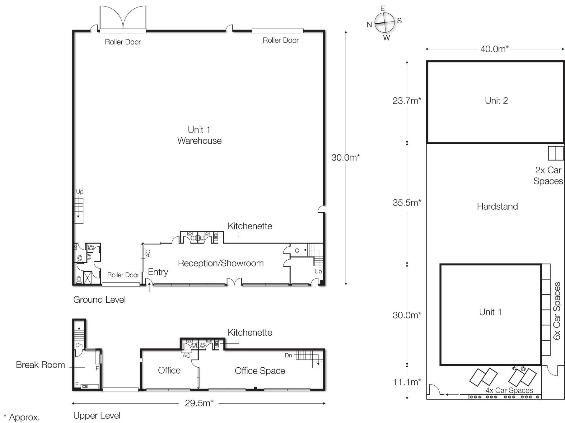
UNIT 1 FLOOR PLAN
